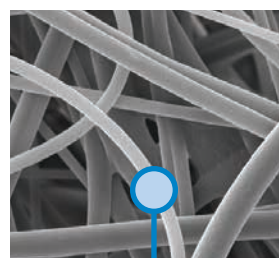
10 Micron Meltblown Media (600x)
