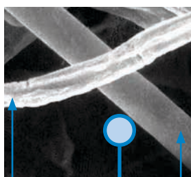
10 Micron Cellulose / Synthetic Media Blend (600x)
