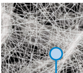
10 Micron Fine Fiber Technology (600x)
